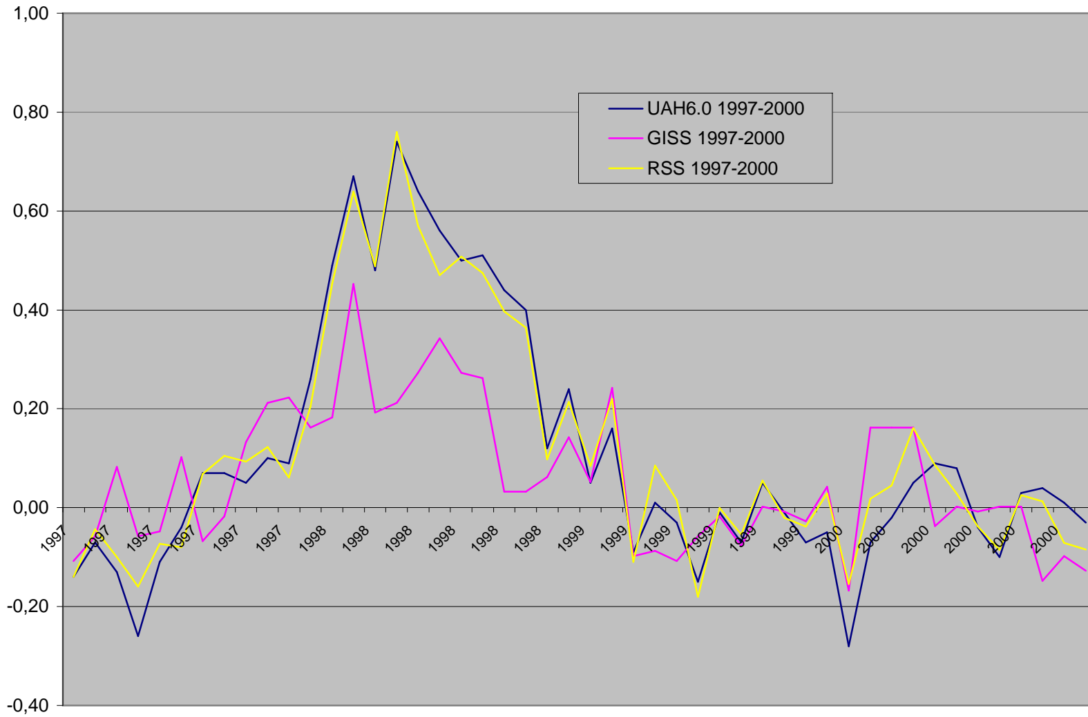
°C Anomaly comparisons: UAH6.0 GISS RSS 1997-2000
